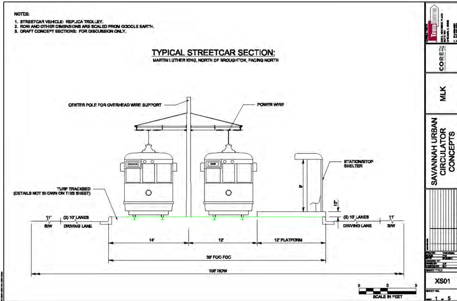
Figure 27. Typical Section – Martin Luther King, Jr. Boulevard
