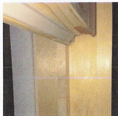
Side Jamb detail with Hidden Balance
