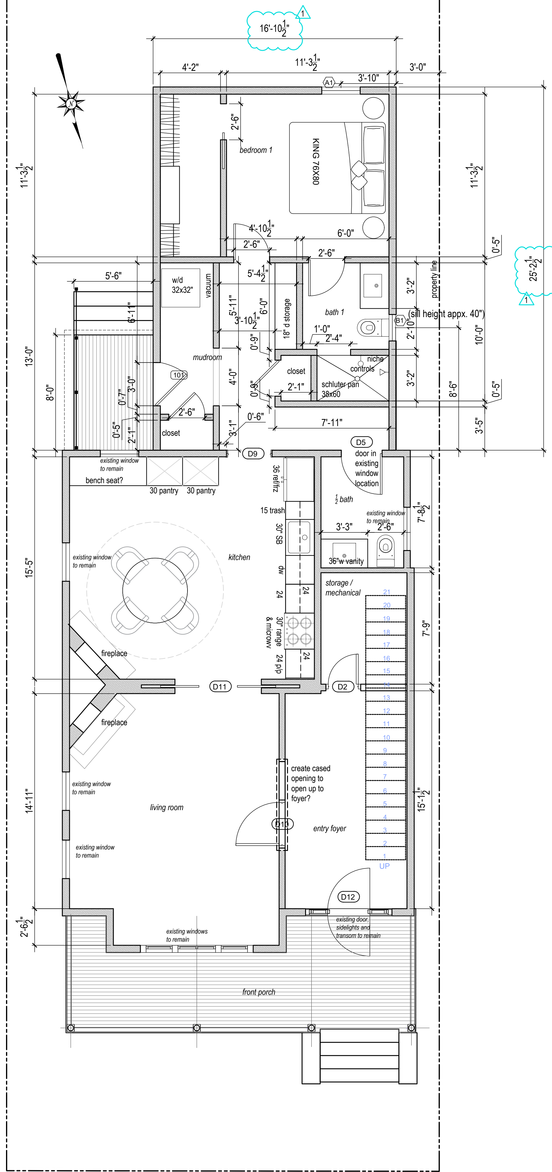
1 PROPOSED FLOOR PLAN: GROUND LEVEL SCALE: 1/4" = 1'-0"
